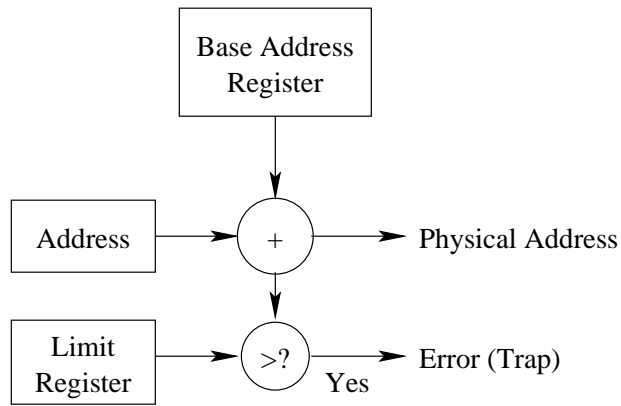
Figure 1. Simple Relocation
