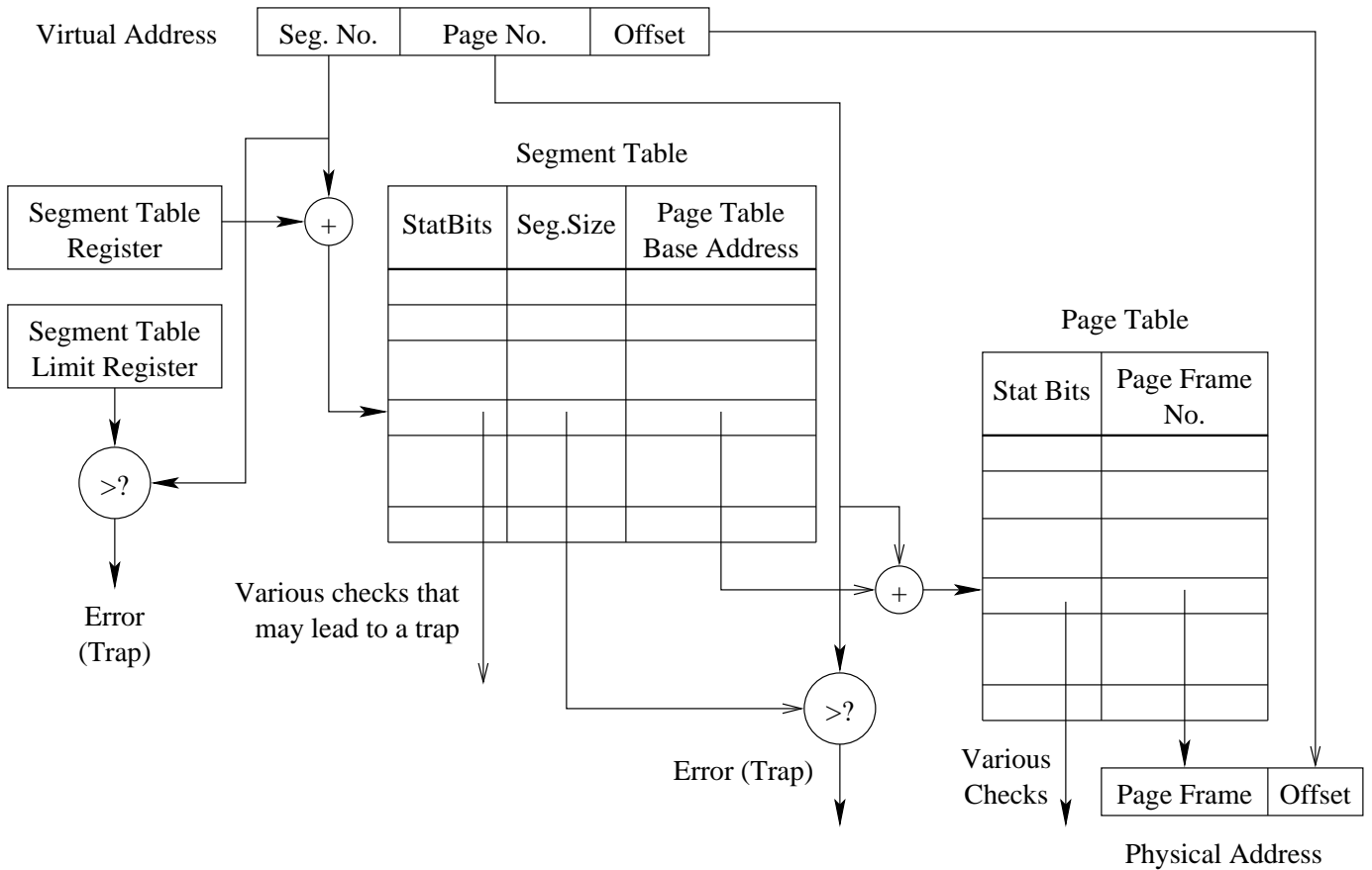
Figure 4. Paged Segments
