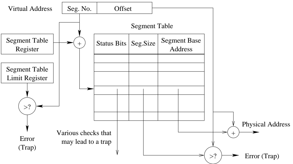
Figure 2. Pure Segments
